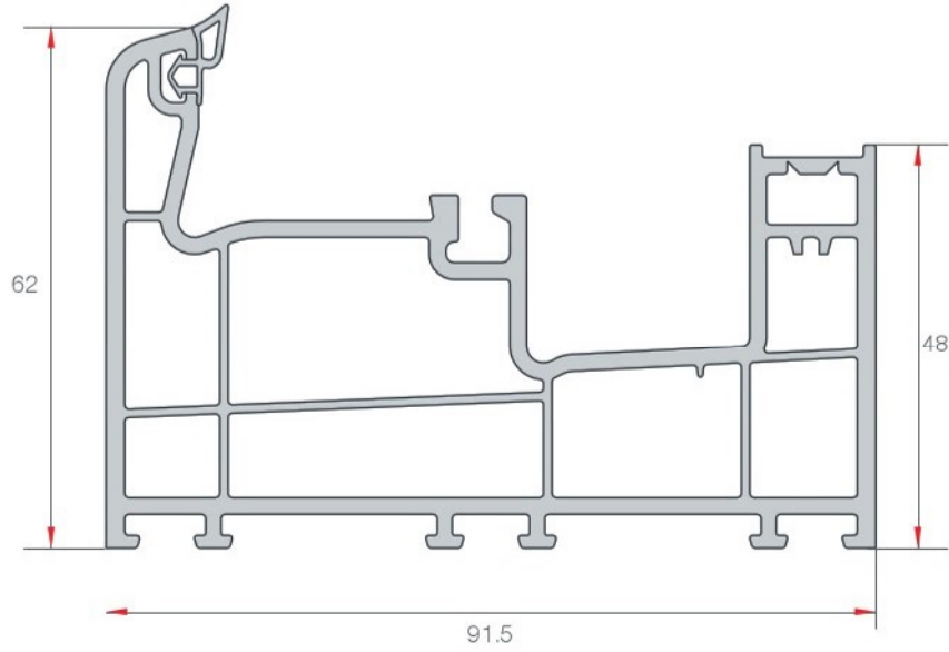
TEK RAYLI SÜRME KASA PROFİLİ SINGLE RAILED SLIDING FRAME PROFILE EN 93 1.425 gr/m
