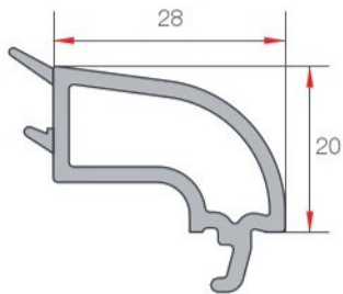
20 mm. OVAL CAM ÇİTASI 20 mm. OVAL GLAZING BEAD EN 106 0.265 gr/m
